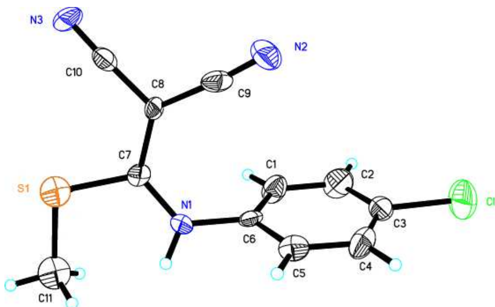
Figure 3. The molecular structure of 2a with 50% probability displacement ellipsoids.
